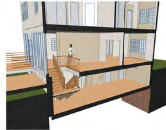
Sectional Elevation
